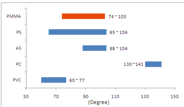
Heat distortion temperature (ASTM D648)
