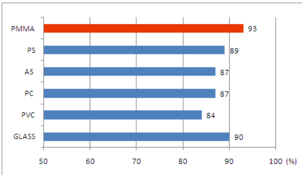
Light transmission (ASTM D1003)
