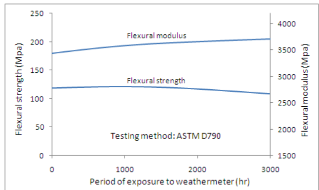
PMMA flexural properties in accelerated exposure
