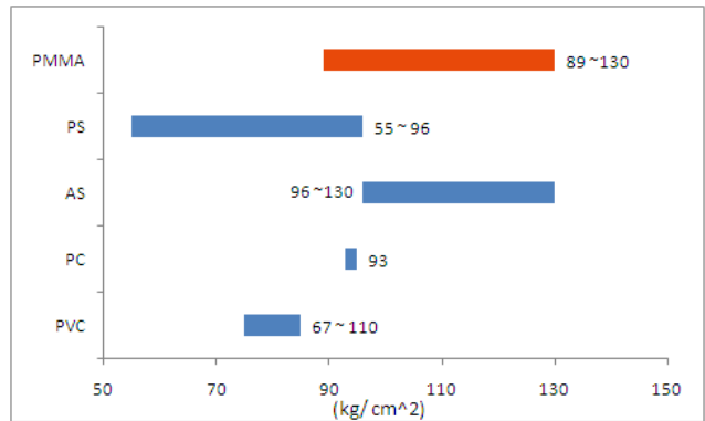
Flexural strength (ASTM D790)
