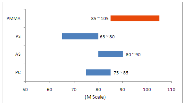
Rockwell hardness (ASTM D785)
