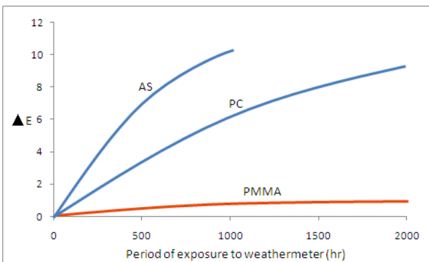
Weatherability - Typical color changes
